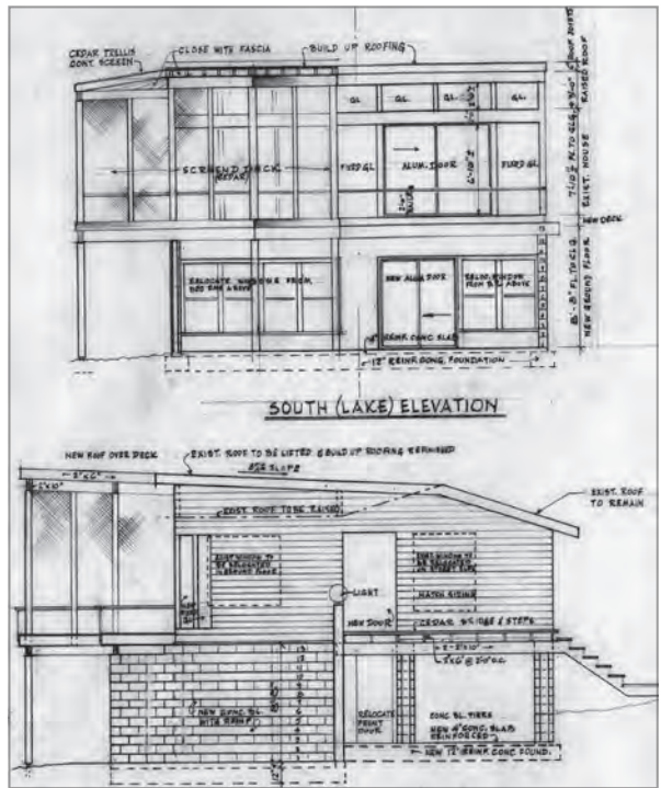
Bergman Street Residence, Austin, TX. East & South Elevations, c. 1973
