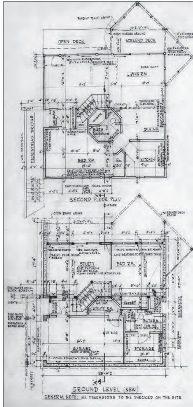
Bergman Street Residence, Austin, TX. Ground & Second Floor Plan, c. 1973
